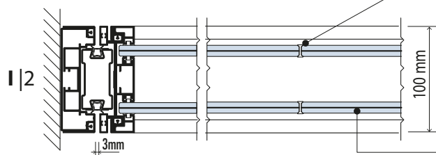
"C-C"
