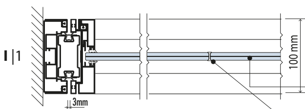
"B-B"
